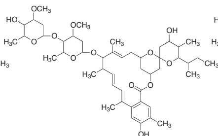
6,8a-seco-6,8a-deoxy-2,5-anhydro AVM B2a
